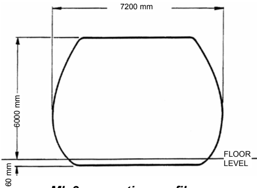
Mk 3 excavation profile
