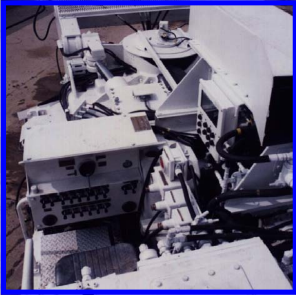
Mk 3 drivers control panel
